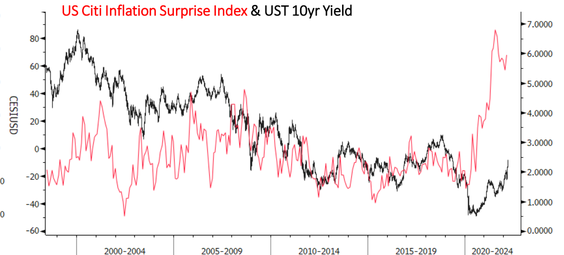
02-Apr-2022 20:42:02 USGG10YR Index (US Generic Govt 10 Yr) US CESI Inf 10yr yield Daily 02JUN1998-23MAR2022
