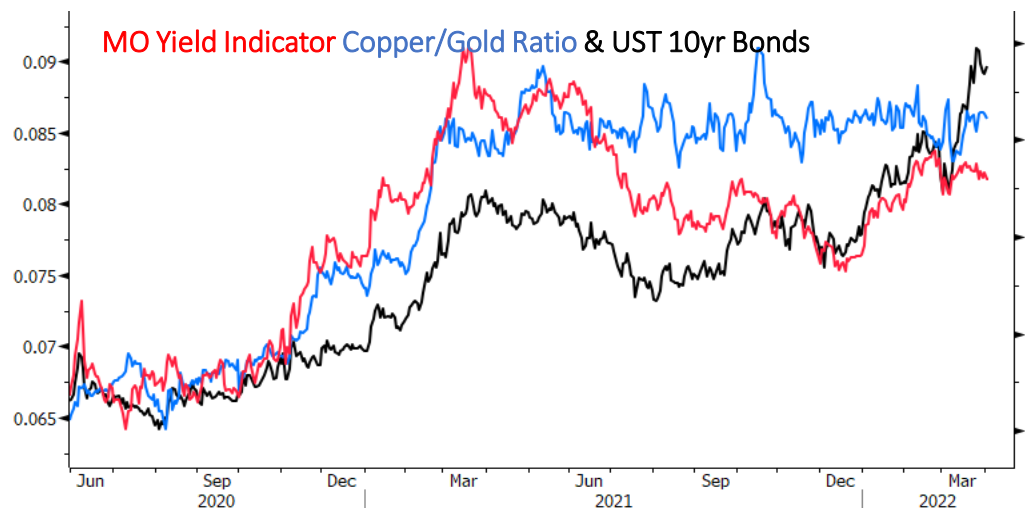
GSTHUSTY Index (Interest Rate Sensitive) rate sensitive vs yield Daily 29MAY2020-03APR2022 Copyright© 2022 Bloomberg Finance L.P. 02-Apr-2022 20:42:29
